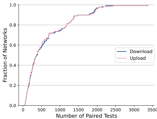
Fig. B.8. CDF of the number of paired tests across all tested networks
