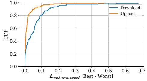
Fig. 12. Distribution of difference in median normalized speed between the best and worst Ookla server across households.
