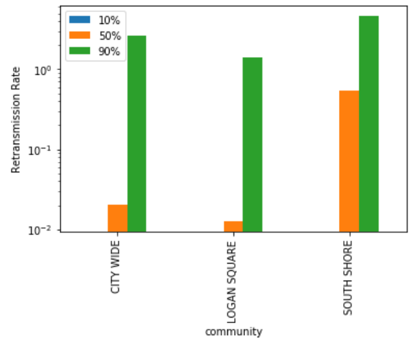
Figure 11: Retransmissions.
