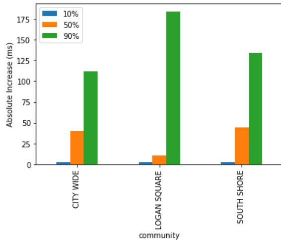
(b) TCP.
